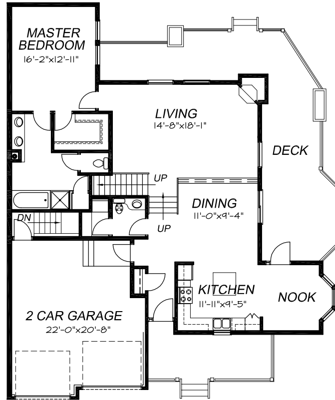
MAIN FLOOR 1,510 SF SECOND FLOOR 718 SF
